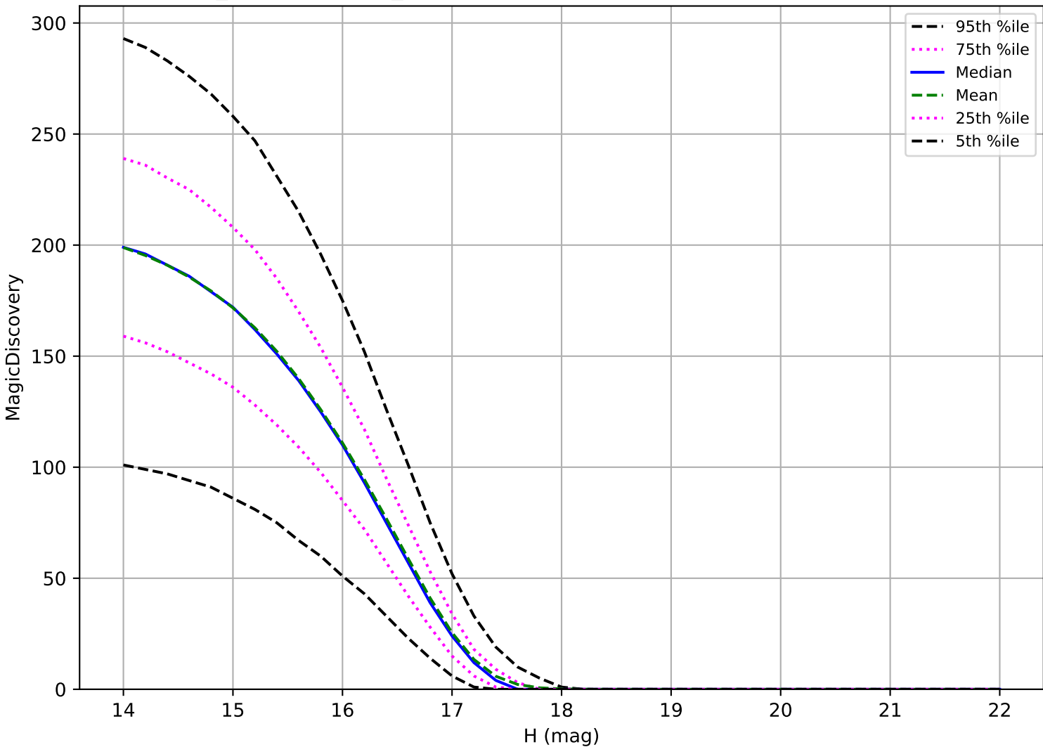
weather_cloudso12v3.4_10yrs: Trojan 6 detections in 60 nights detection loss
