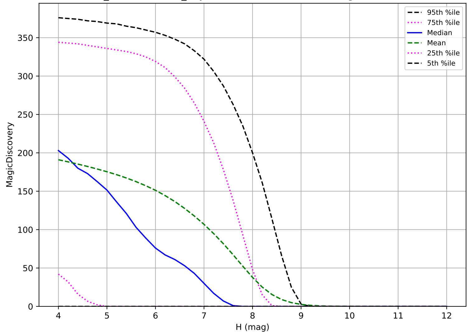
weather_cloudso12v3.4_10yrs: TNO 6 detections in 60 nights detection loss
