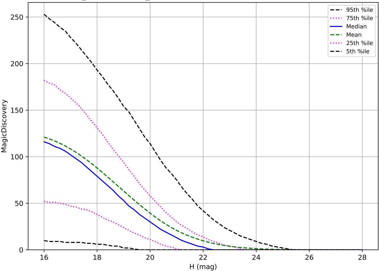
weather_cloudso12v3.4_10yrs: PHA 6 detections in 60 nights detection loss
