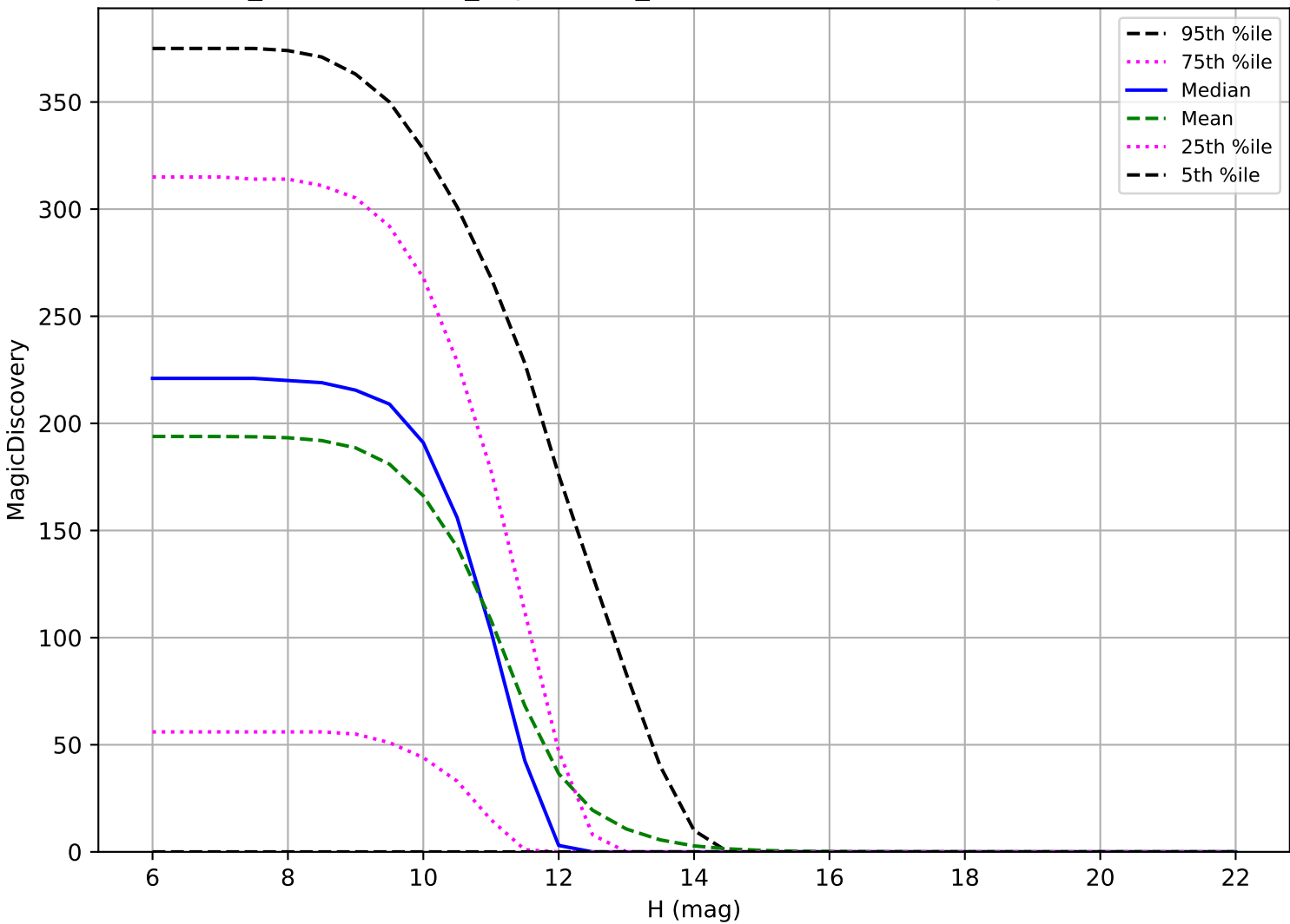
weather_cloudso12v3.4_10yrs: OCC_r20 6 detections in 60 nights detection loss
