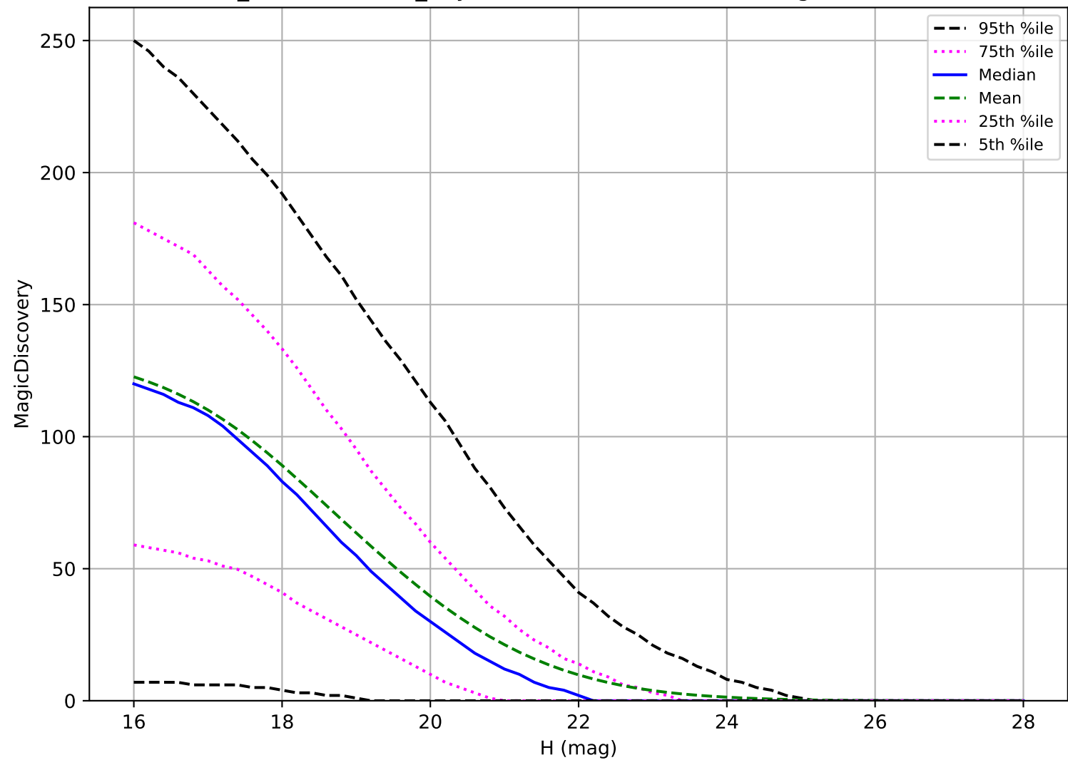
weather_cloudso12v3.4_10yrs: NEO 6 detections in 60 nights detection loss
