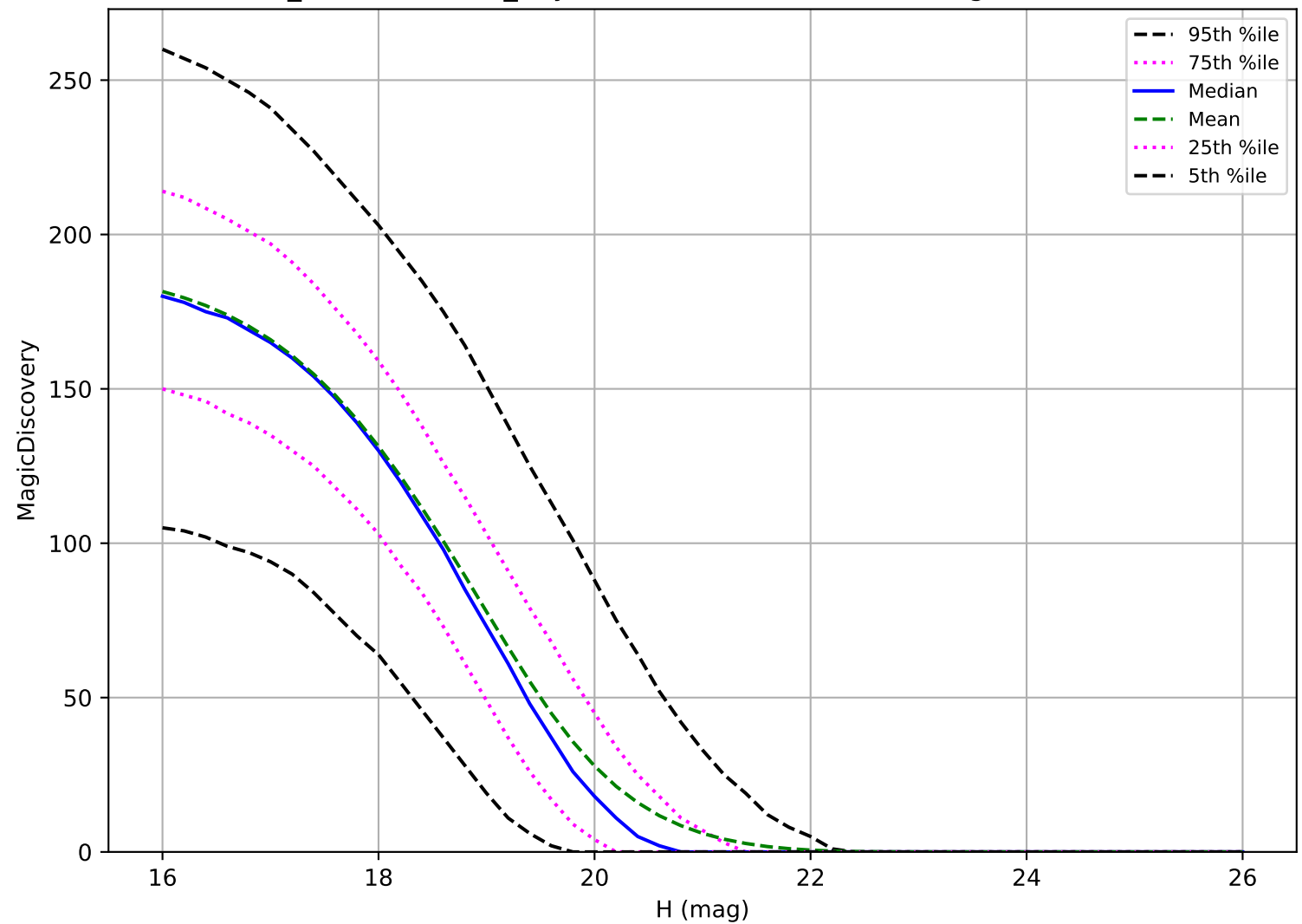
weather_cloudso12v3.4_10yrs: MBA 6 detections in 60 nights detection loss
