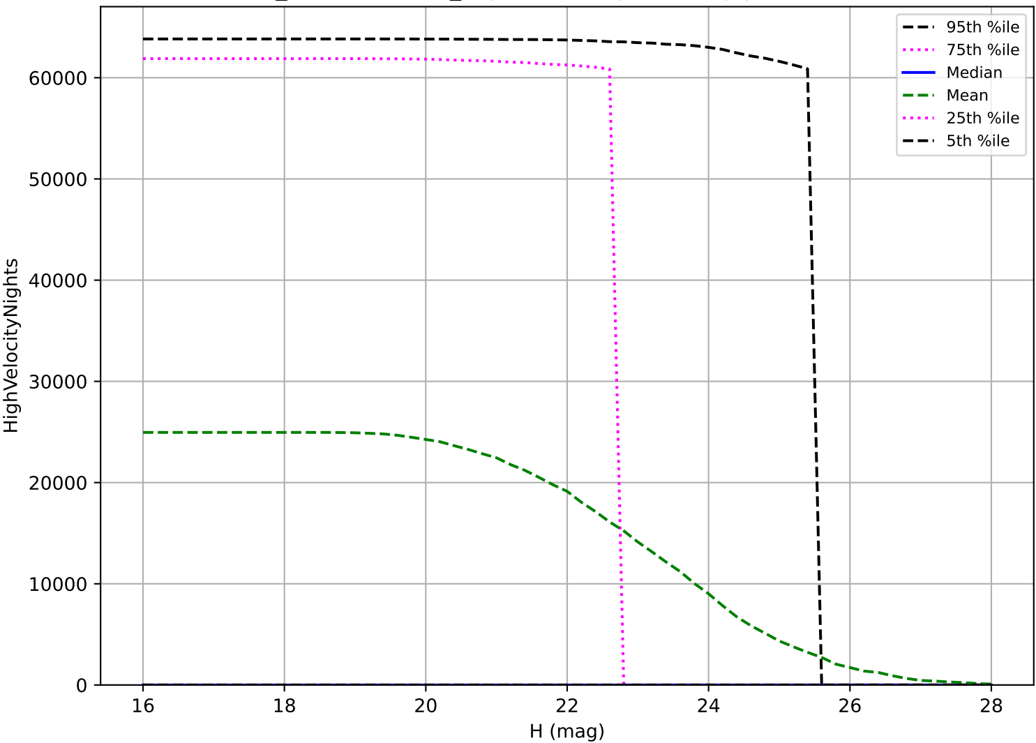
weather_cloudso12v3.4_10yrs: PHA High velocity pair detection loss
