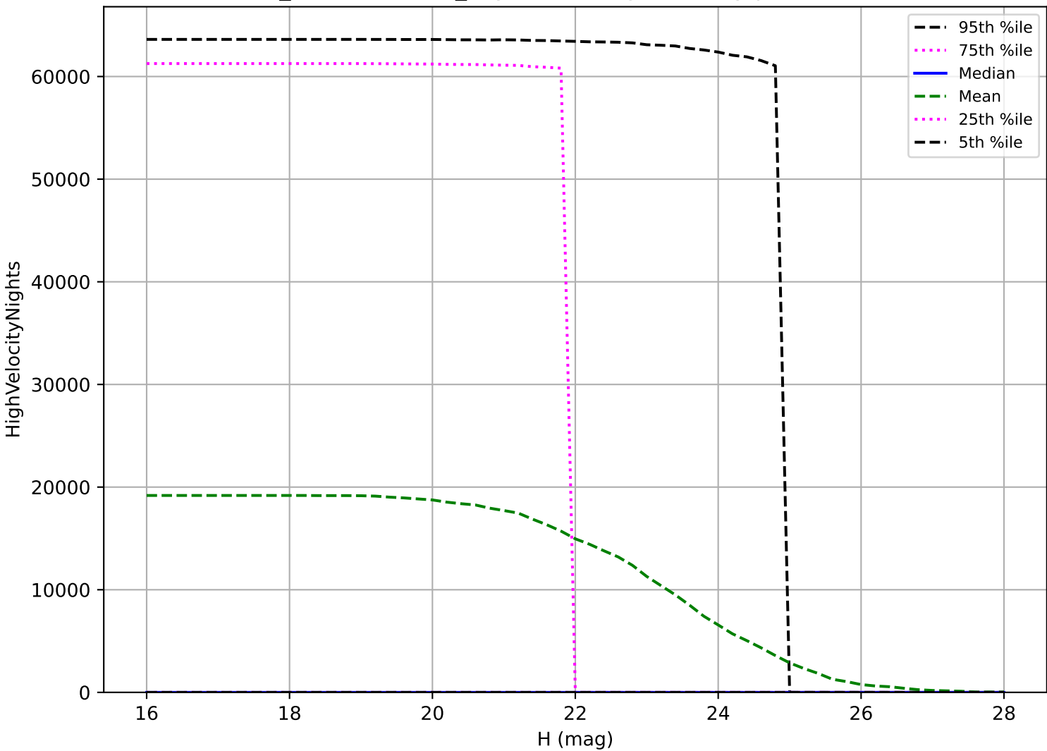
weather_cloudso12v3.4_10yrs: NEO High velocity pair detection loss
