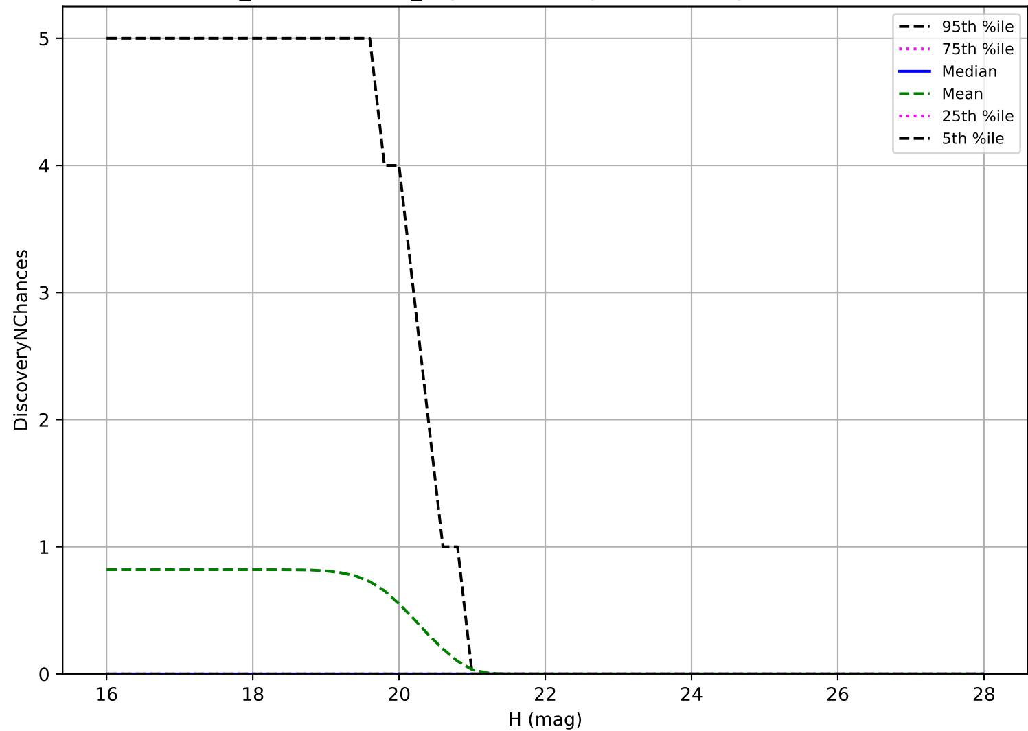
weather_cloudso12v3.4_10yrs: Vatira 3 pairs in 15 nights detection loss
