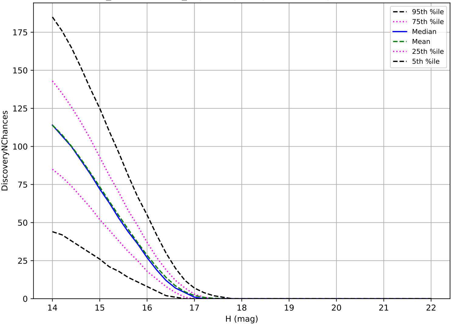
weather_cloudso12v3.4_10yrs: Trojan 3 pairs in 15 nights detection loss
