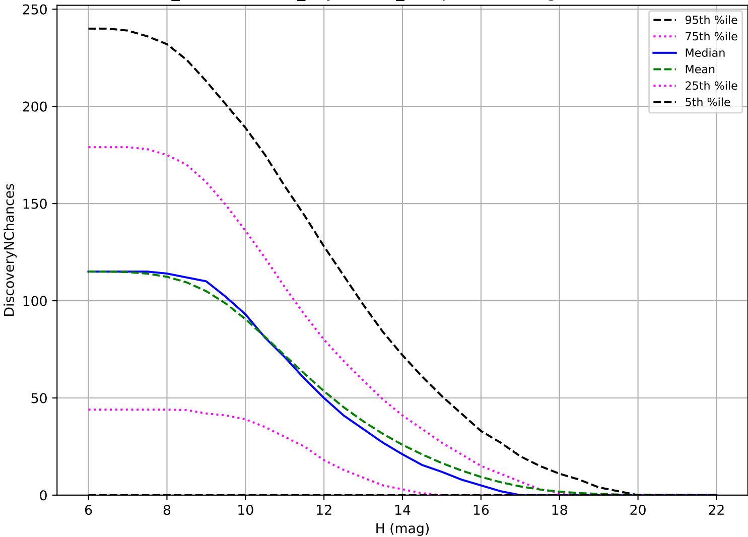
weather_cloudso12v3.4_10yrs: OCC_r5 3 pairs in 15 nights detection loss
