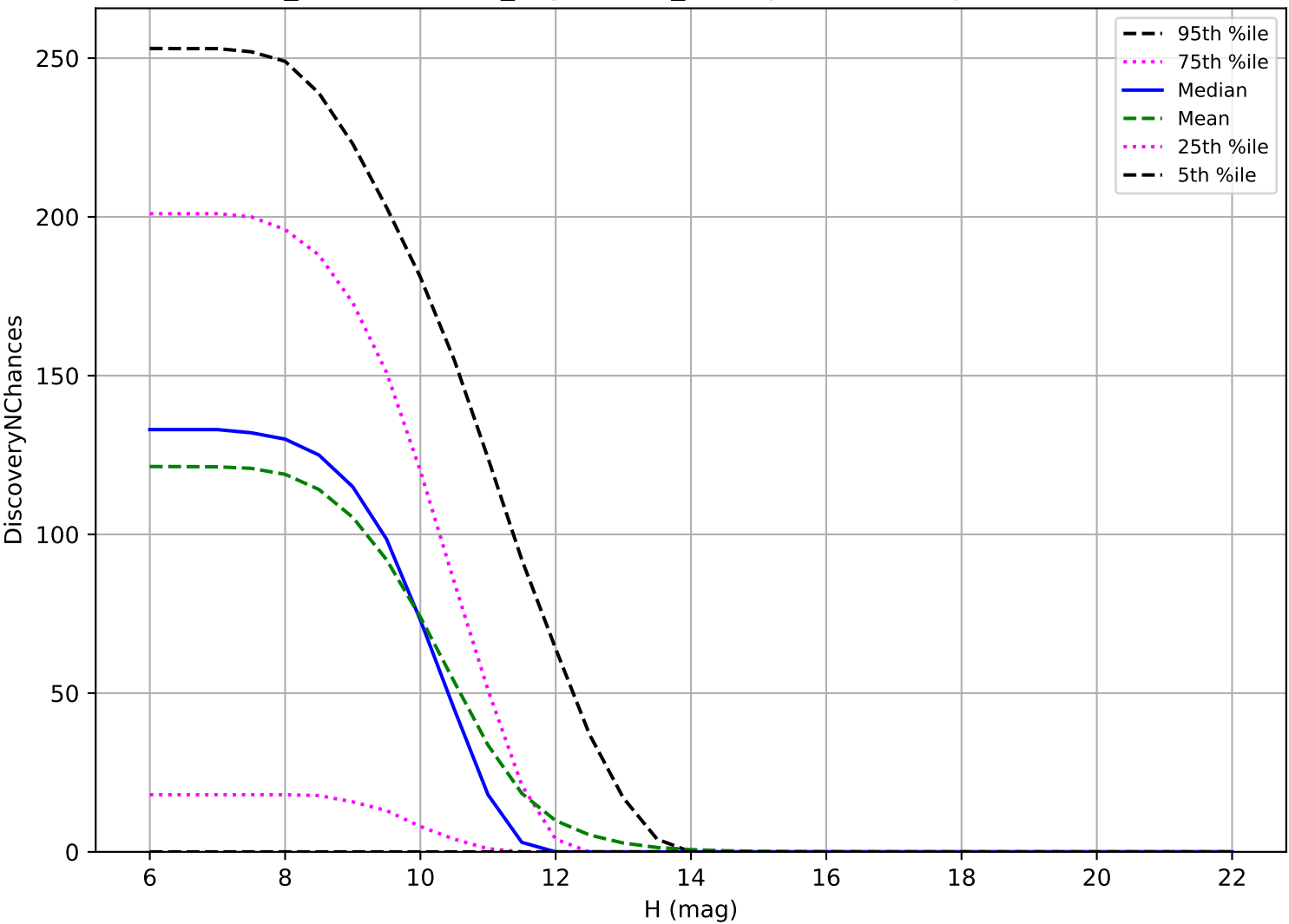
weather_cloudso12v3.4_10yrs: OCC_r20 3 pairs in 15 nights detection loss
