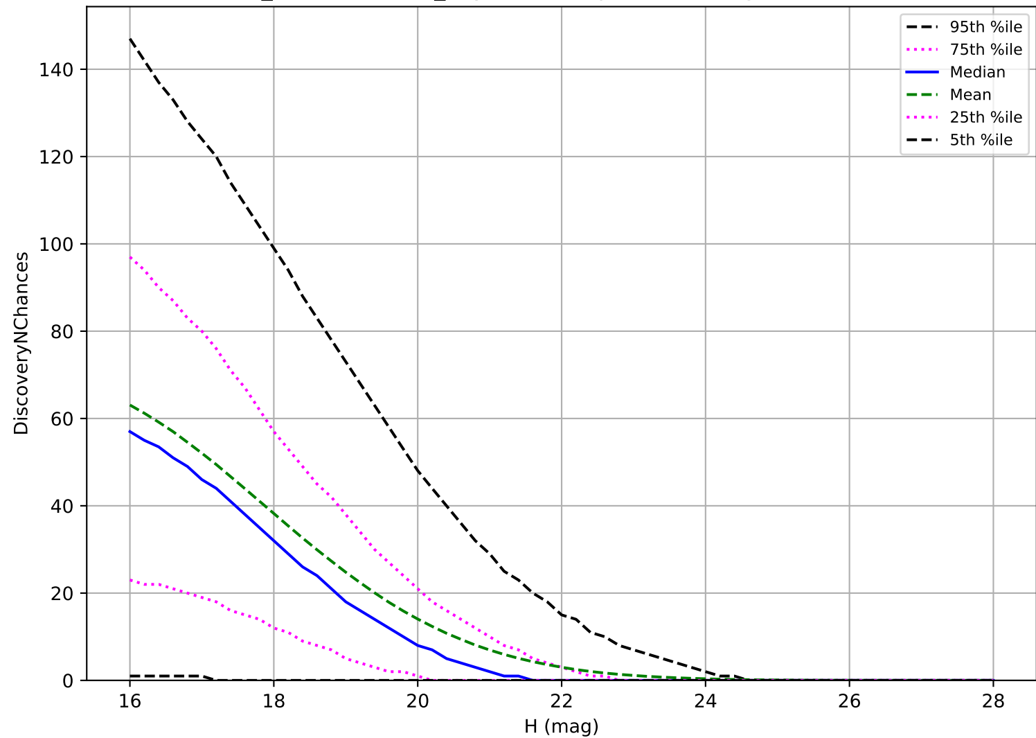
weather_cloudso12v3.4_10yrs: NEO 3 pairs in 15 nights detection loss
