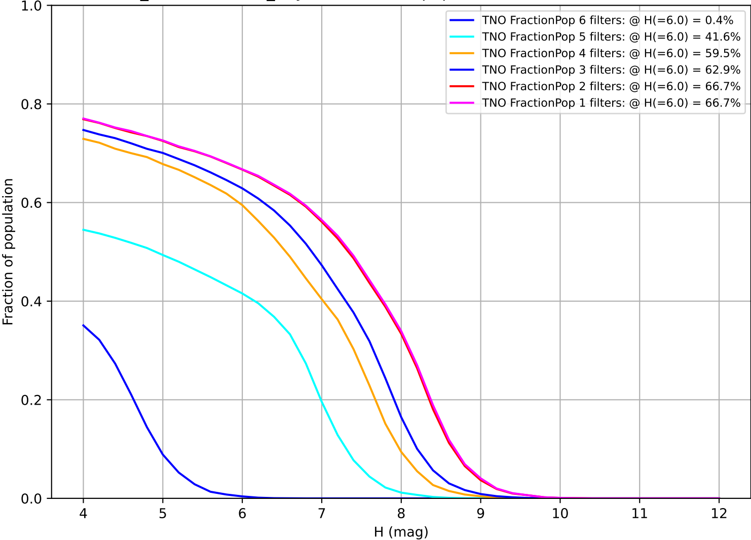
weather_cloudso12v3.4_10yrs: Fraction of population with colors in X filters TNO
