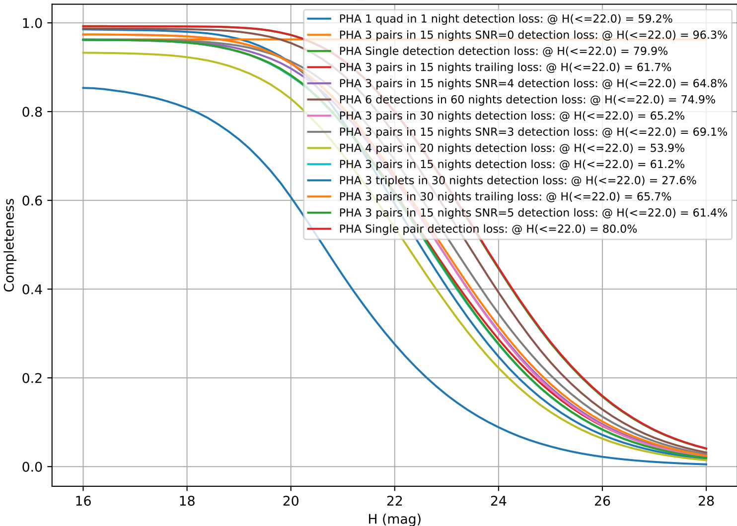
weather_cloudso12v3.4_10yrs: CumulativeCompleteness
