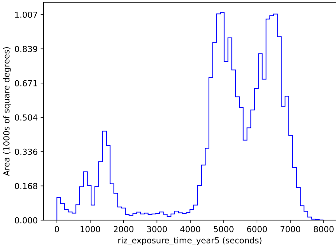
weather_cloudso12v3.4_10yrs gri band non-DD: riz_exposure_time_year5
