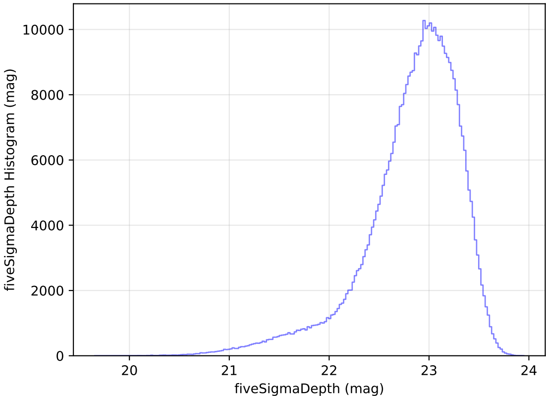
weather_cloudso12v3.4_10yrs z: fiveSigmaDepth Histogram
