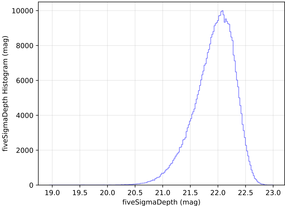
weather_cloudso12v3.4_10yrs y: fiveSigmaDepth Histogram
