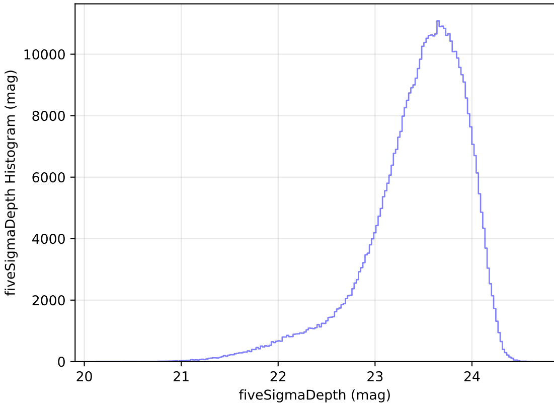
weather_cloudso12v3.4_10yrs i: fiveSigmaDepth Histogram
