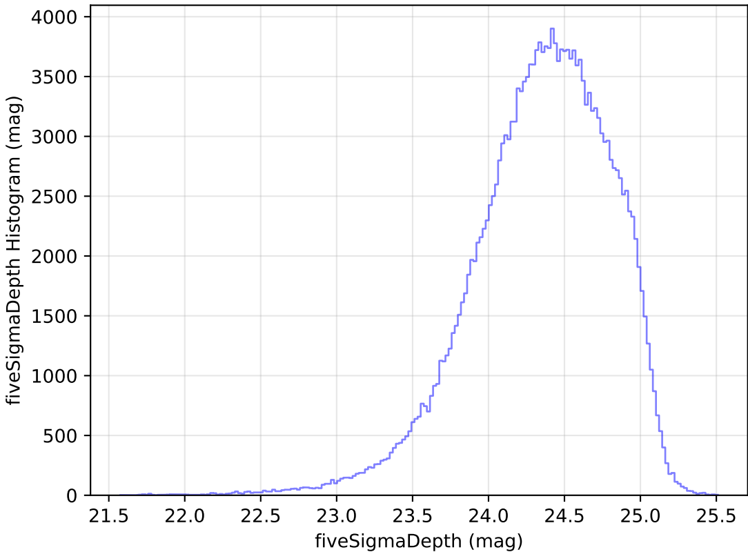
weather_cloudso12v3.4_10yrs g: fiveSigmaDepth Histogram
