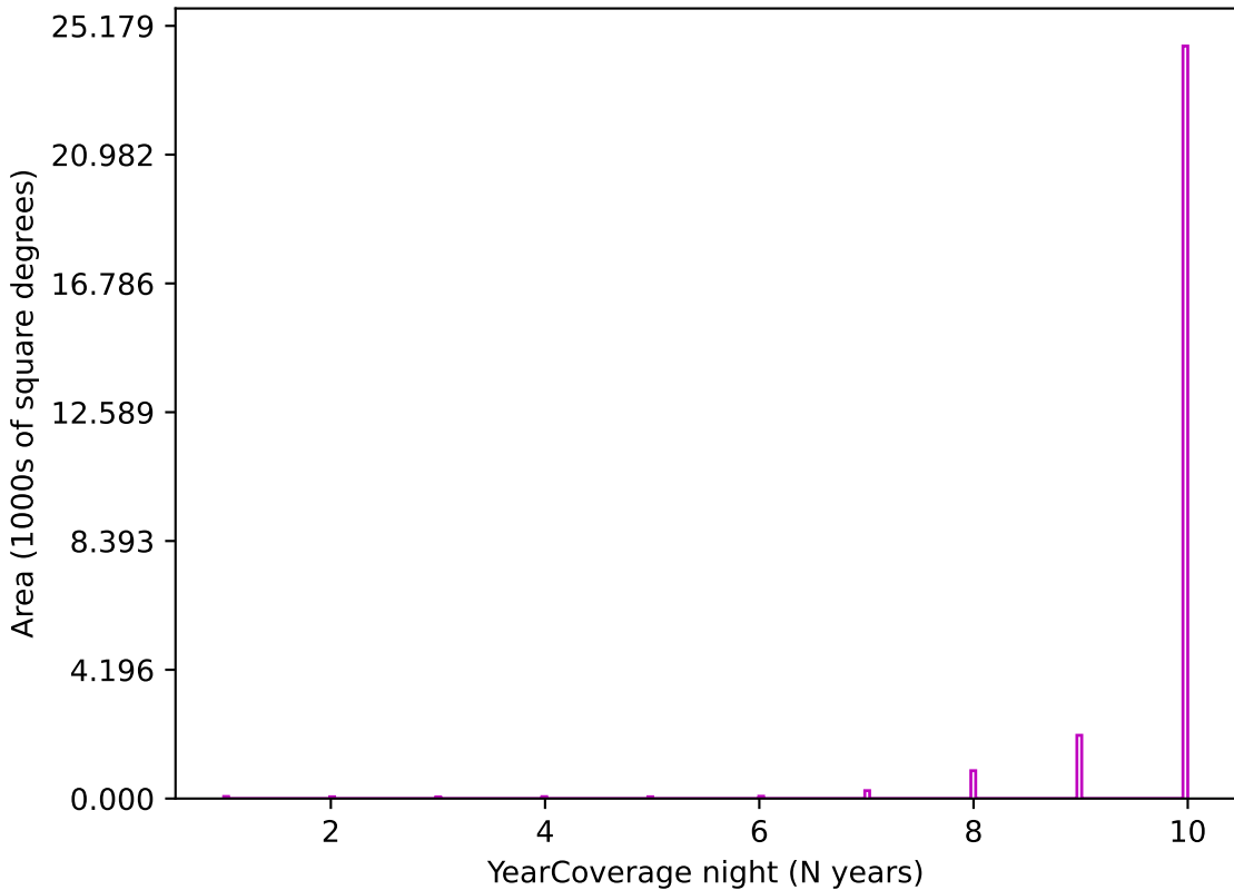
weather_cloudso12v3.4_10yrs z band: YearCoverage night
