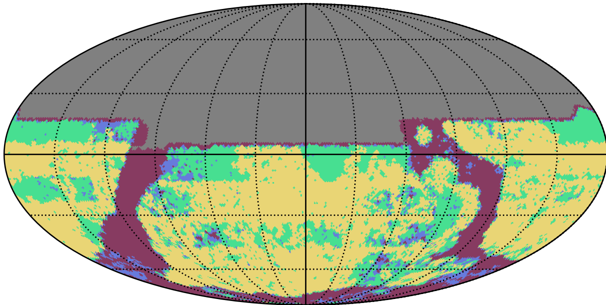
weather_cloudso12v3.4_10yrs u band: YearCoverage night
