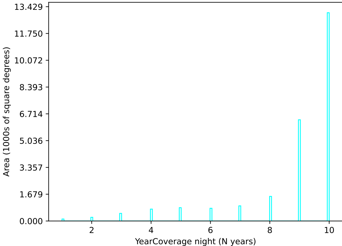
weather_cloudso12v3.4_10yrs u band: YearCoverage night
