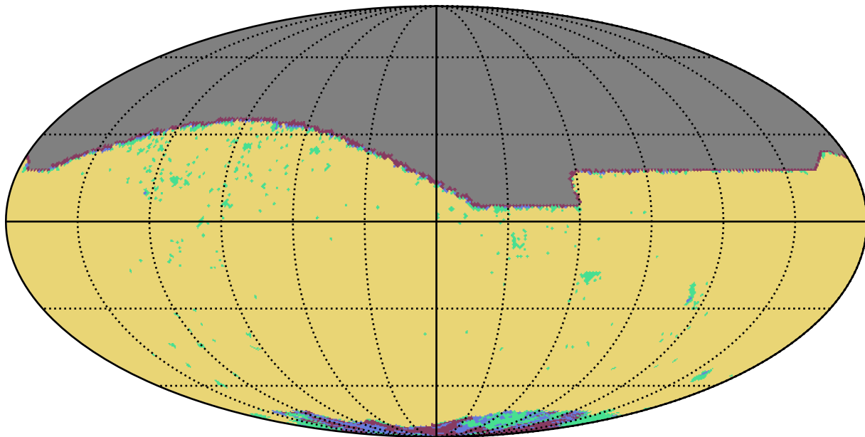
weather_cloudso12v3.4_10yrs r band: YearCoverage night
