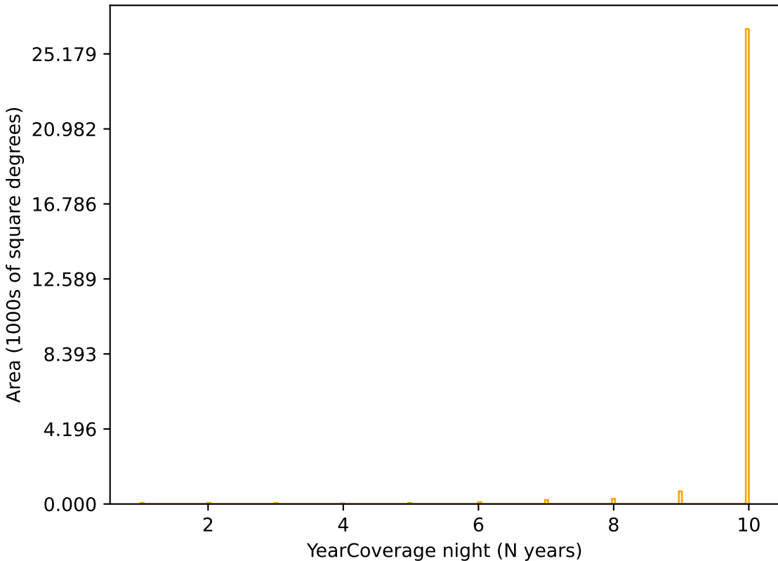
weather_cloudso12v3.4_10yrs r band: YearCoverage night
