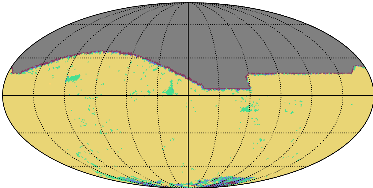
weather_cloudso12v3.4_10yrs i band: YearCoverage night
