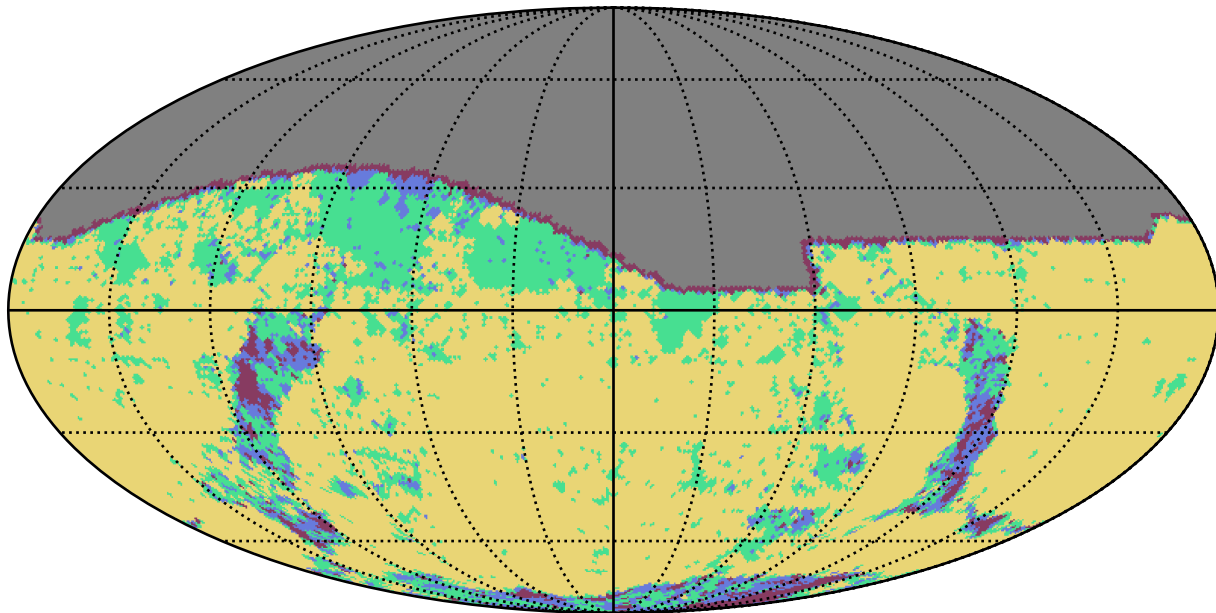
weather_cloudso12v3.4_10yrs g band: YearCoverage night
