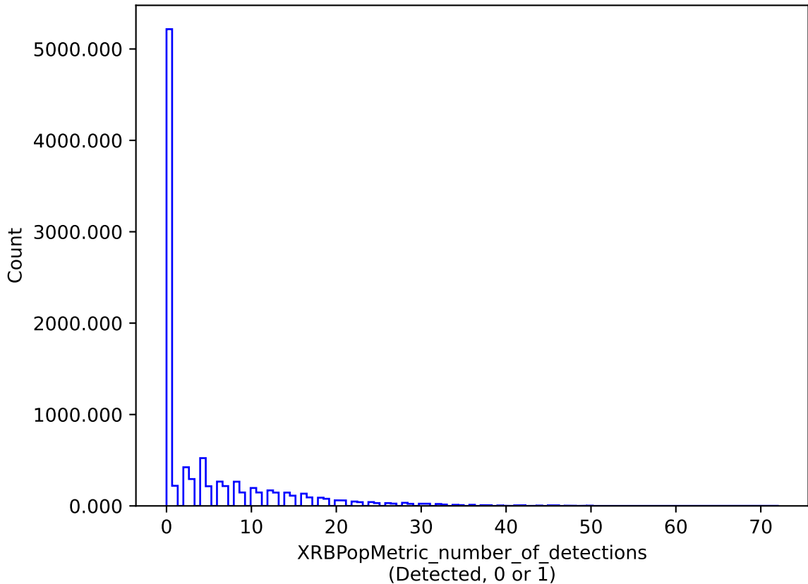
weather_cloudso12v3.4_10yrs : XRBPoMetric_number_of_detections
