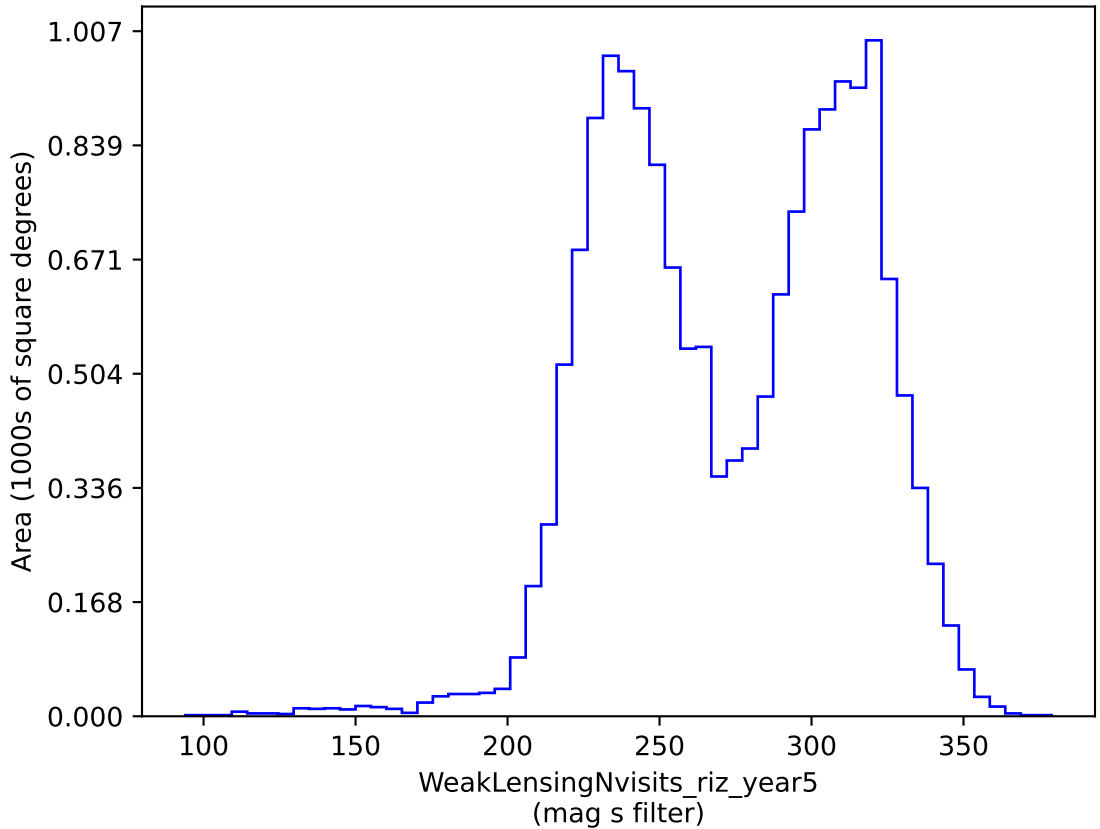
weather_cloudso12v3.4_10yrs gri band non-DD: WeakLensingNvisits_riz_year5
