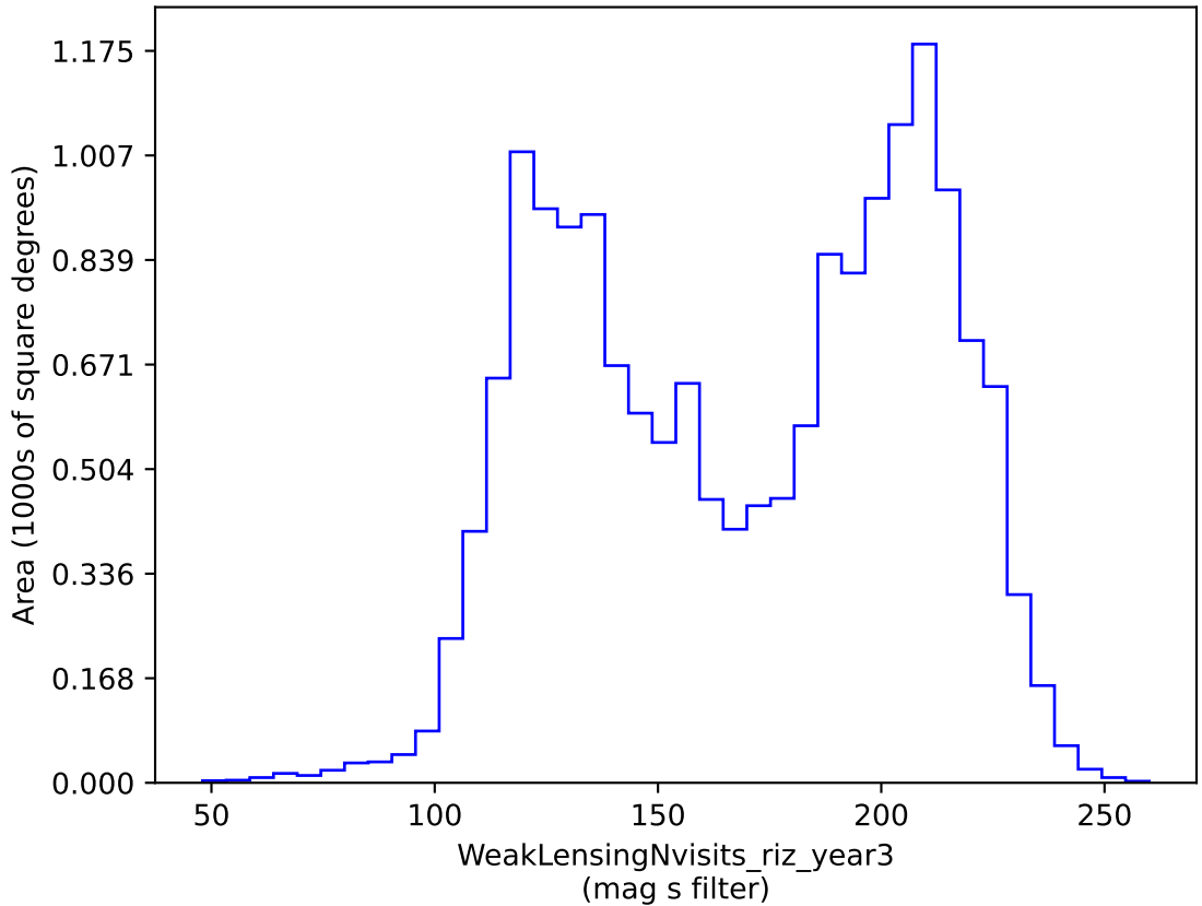
weather_cloudso12v3.4_10yrs gri band non-DD: WeakLensingNvisits_riz_year3
