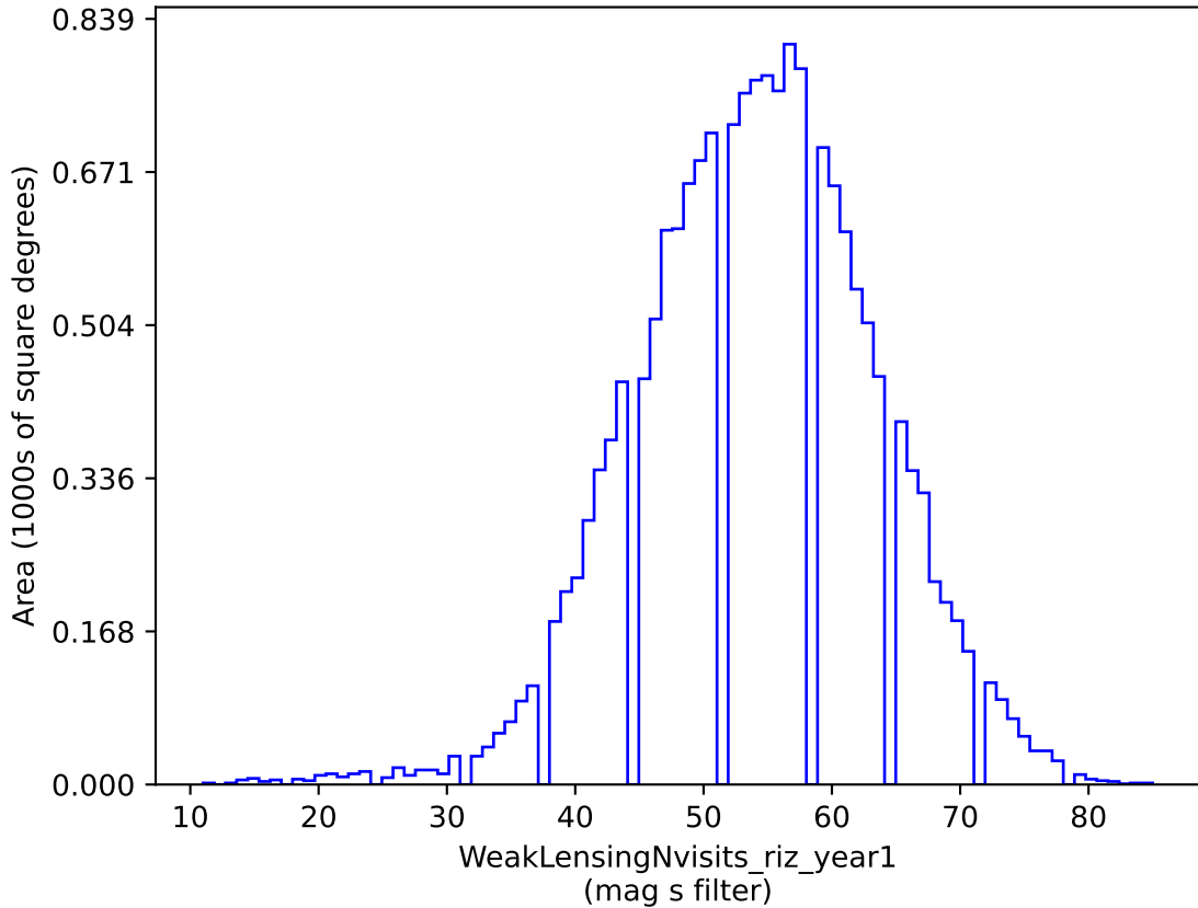
weather_cloudso12v3.4_10yrs gri band non-DD: WeakLensingNvisits_riz_year1
