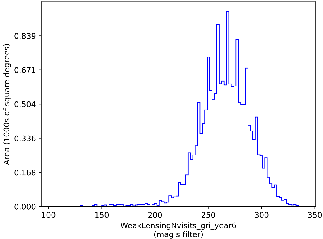
weather_cloudso12v3.4_10yrs gri band non-DD: WeakLensingNvisits_gri_year6
