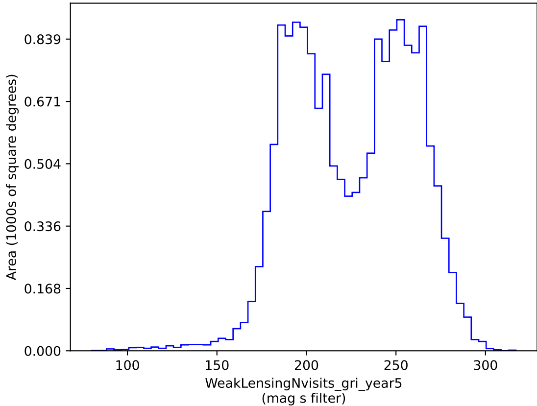
weather_cloudso12v3.4_10yrs gri band non-DD: WeakLensingNvisits_gri_year5
