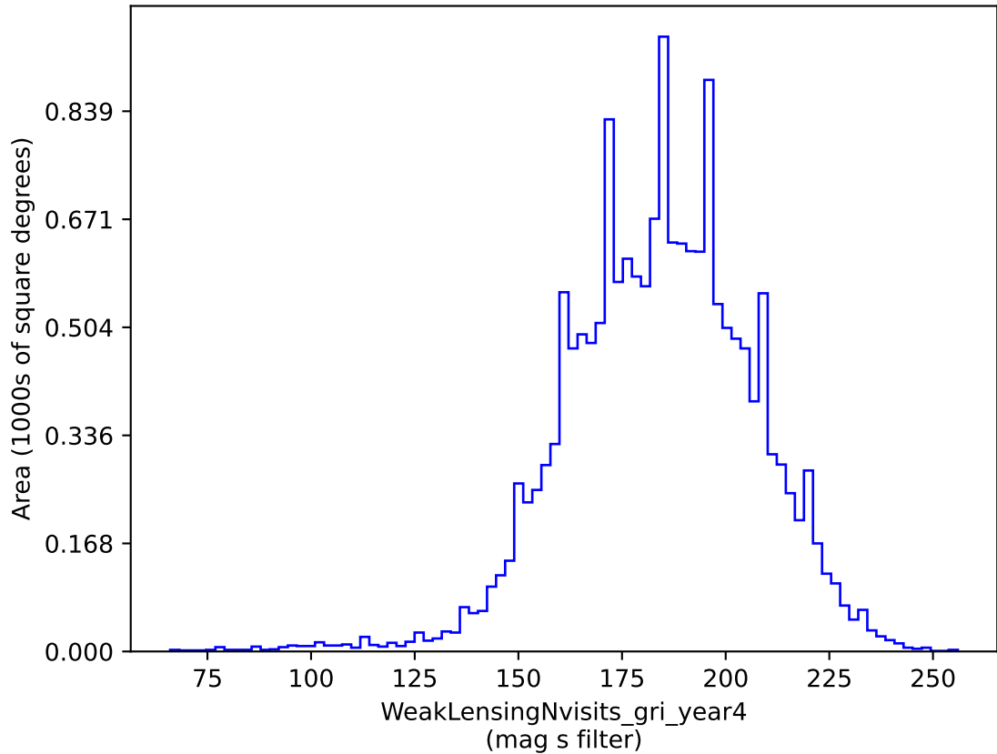
weather_cloudso12v3.4_10yrs gri band non-DD: WeakLensingNvisits_gri_year4
