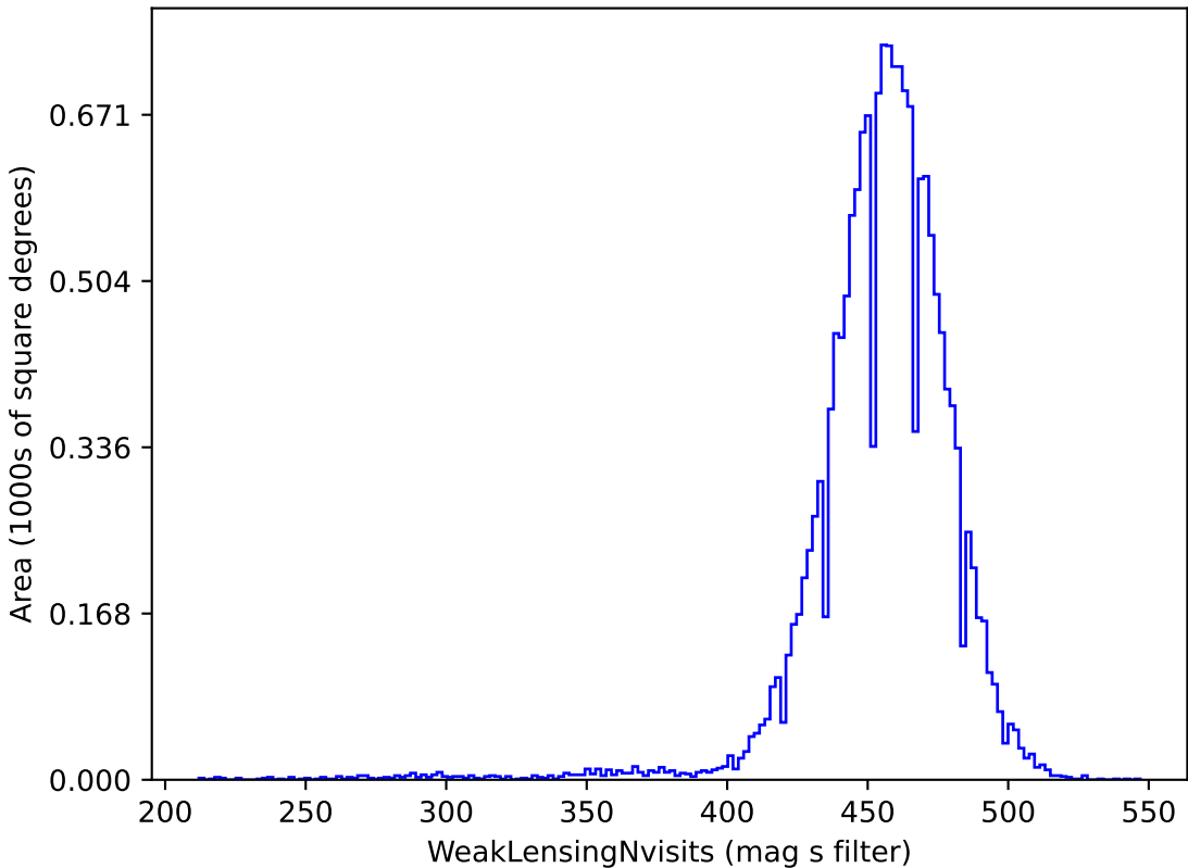
weather_cloudso12v3.4_10yrs gri band non-DD: WeakLensingNvisits
