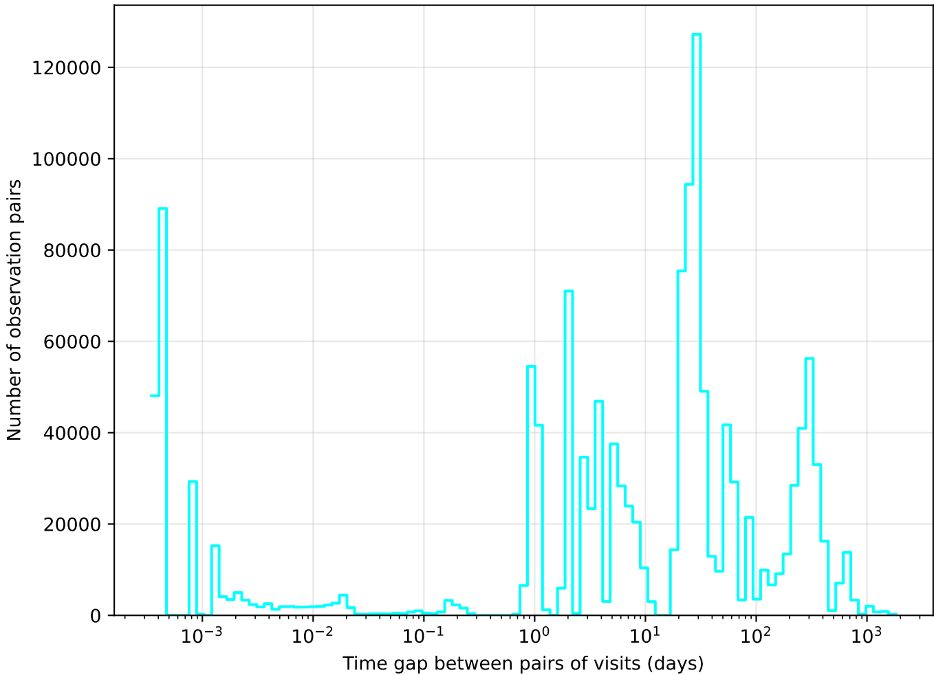
weather_cloudso12v3.4_10yrs u band: Tgaps observationStartMJD
