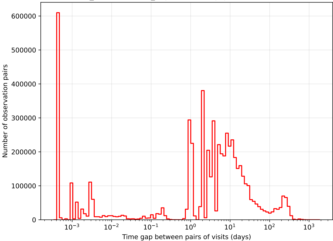
weather_cloudso12v3.4_10yrs i band: Tgaps observationStartMJD
