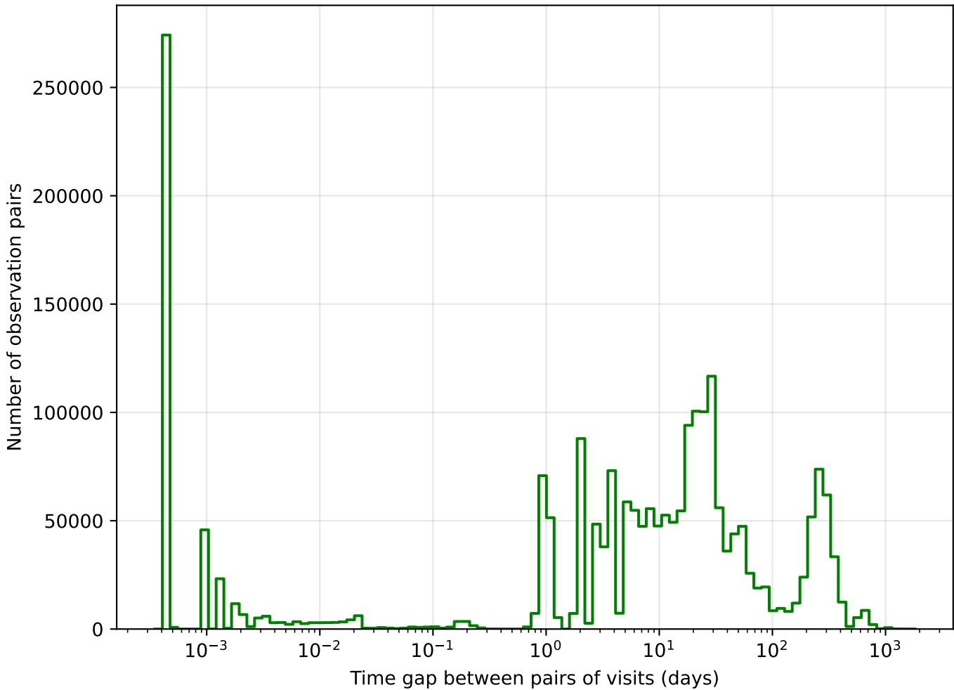
weather_cloudso12v3.4_10yrs g band: Tgaps observationStartMJD
