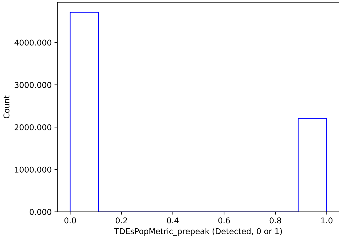
weather_cloudso12v3.4_10yrs : TDEsPopMetric_prepeak
