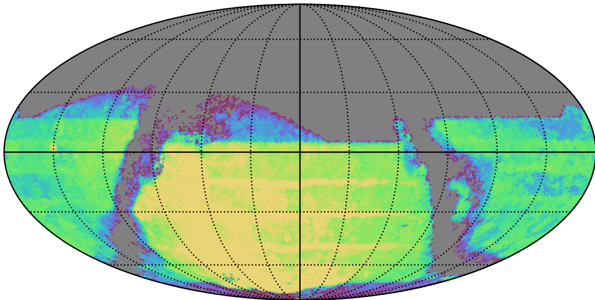
weather_cloudso12v3.4_10yrs : TDC_season
