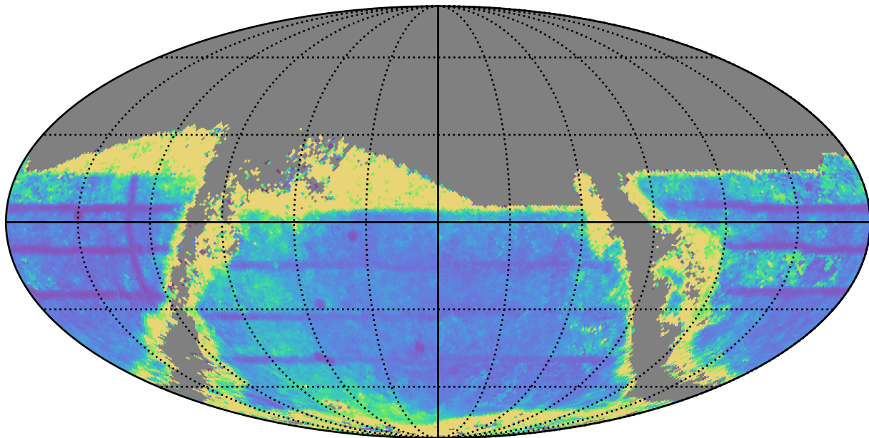
weather_cloudso12v3.4_10yrs : TDC_cadence
