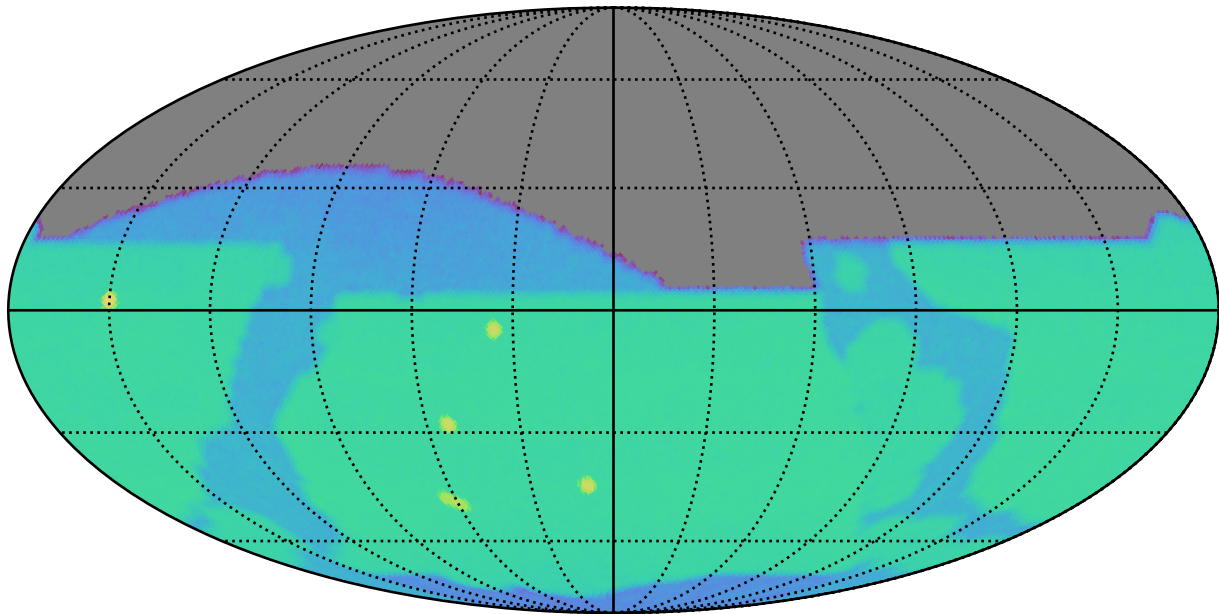
weather_cloudso12v3.4_10yrs z: SurfaceBrightLimit
