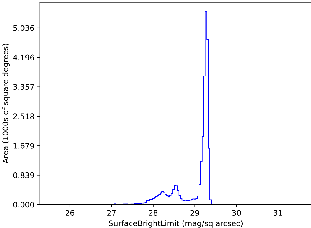
weather_cloudso12v3.4_10yrs z: SurfaceBrightLimit
