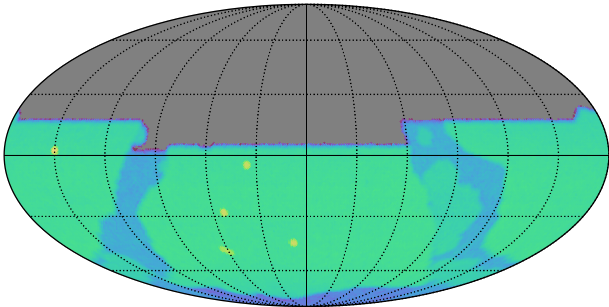
weather_cloudso12v3.4_10yrs y: SurfaceBrightLimit
