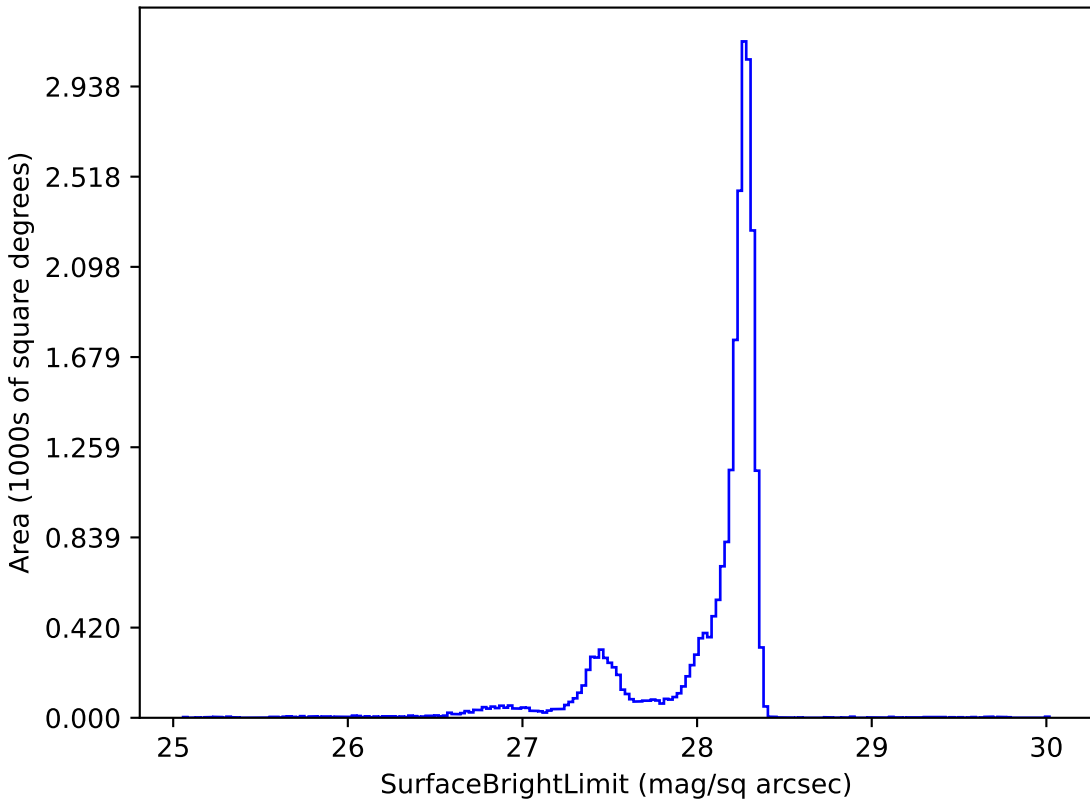
weather_cloudso12v3.4_10yrs y: SurfaceBrightLimit
