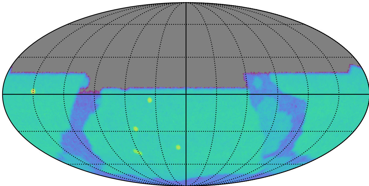
weather_cloudso12v3.4_10yrs u: SurfaceBrightLimit
