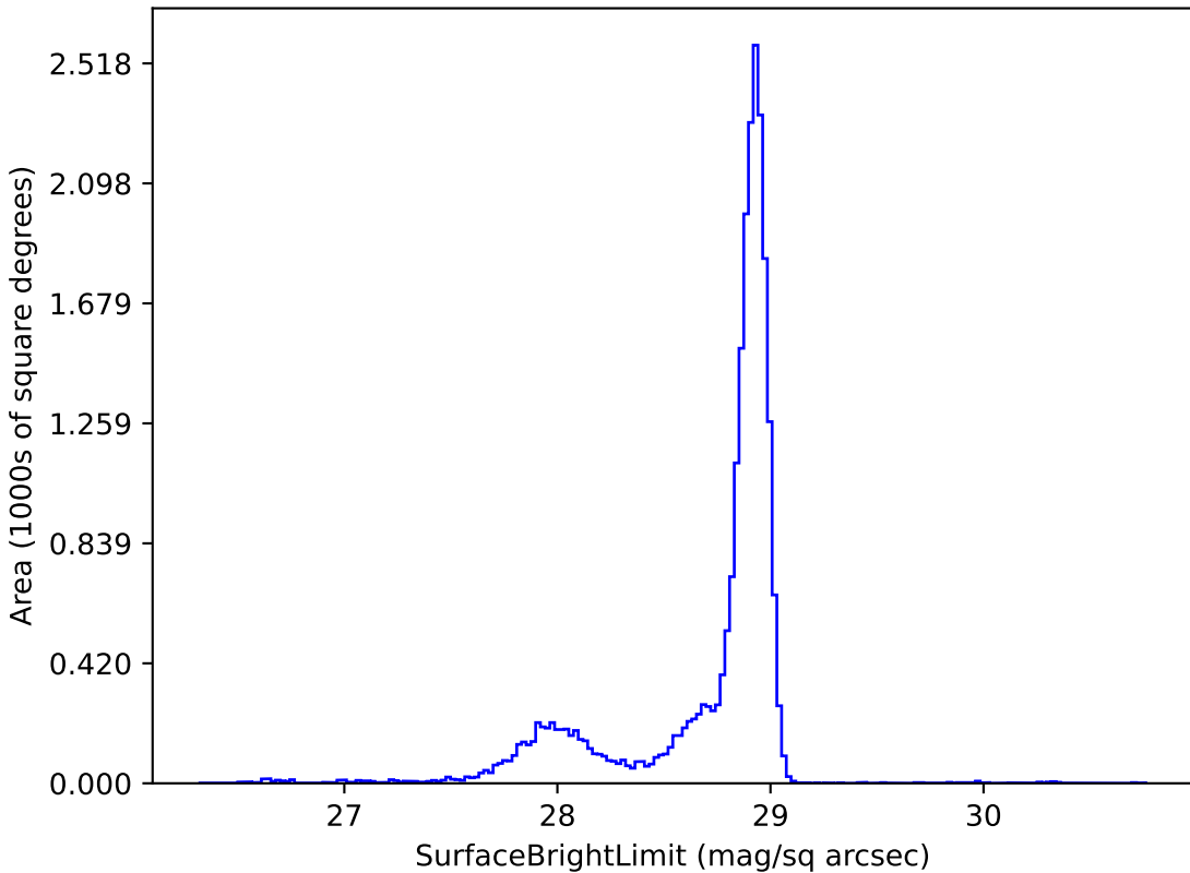
weather_cloudso12v3.4_10yrs u: SurfaceBrightLimit
