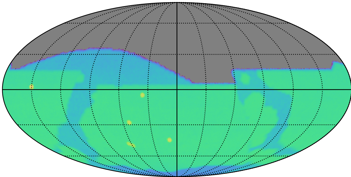
weather_cloudso12v3.4_10yrs r: SurfaceBrightLimit
