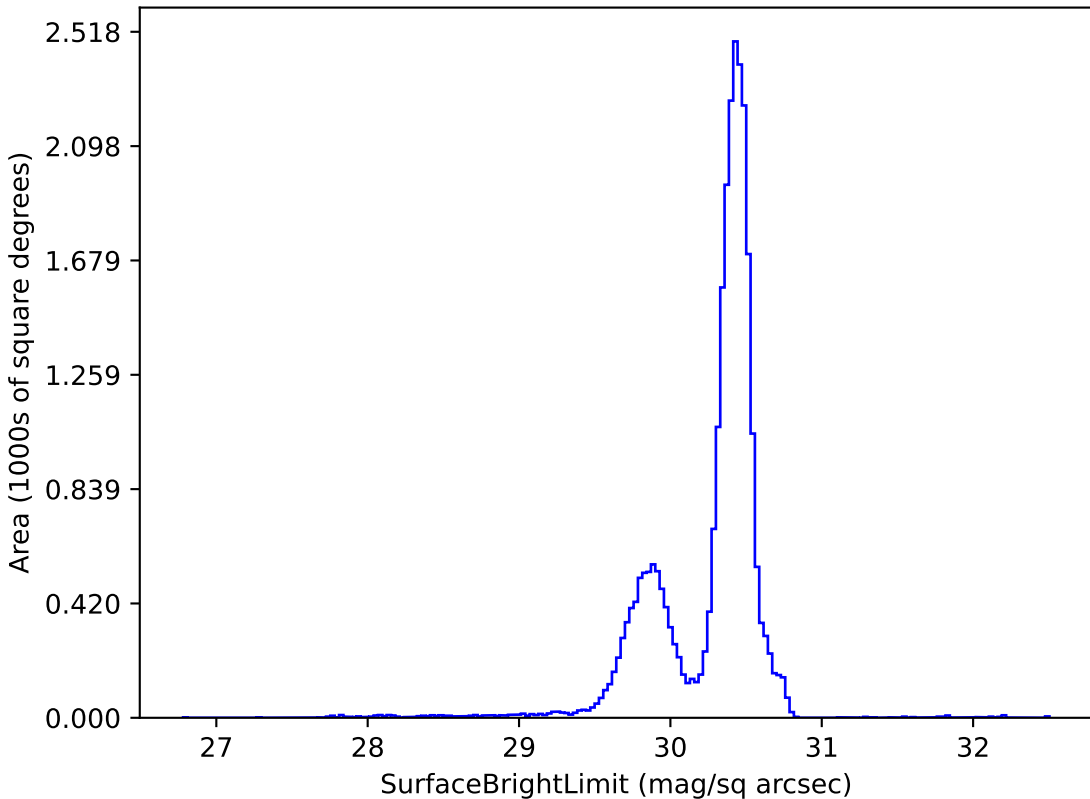
weather_cloudso12v3.4_10yrs g: SurfaceBrightLimit
