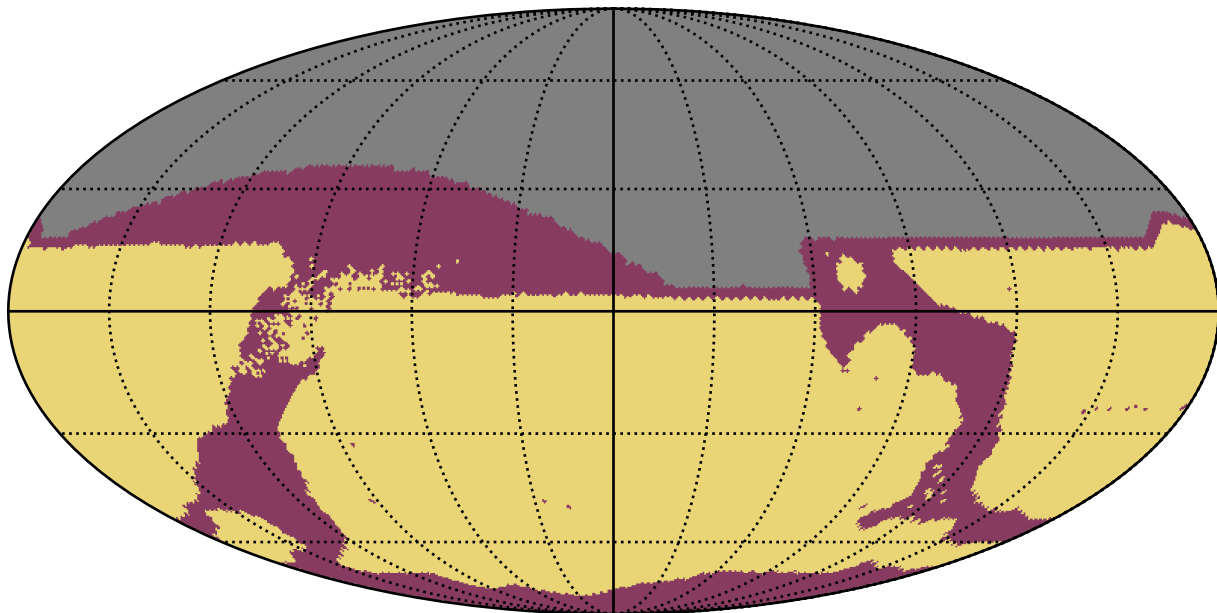
weather_cloudso12v3.4_10yrs : RapidRevisits
